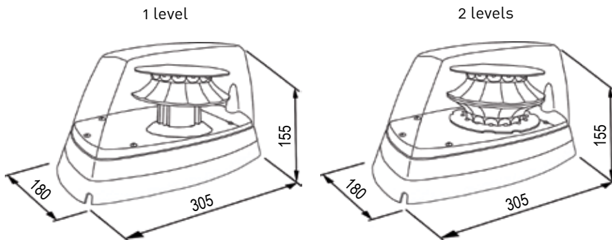
Trident II Solaris dimensions (mm).
