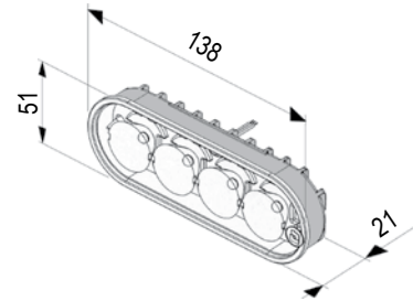
MicroLed Plus dimensions (mm).
