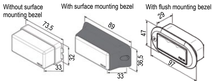
Impaxx dimensions (mm).
