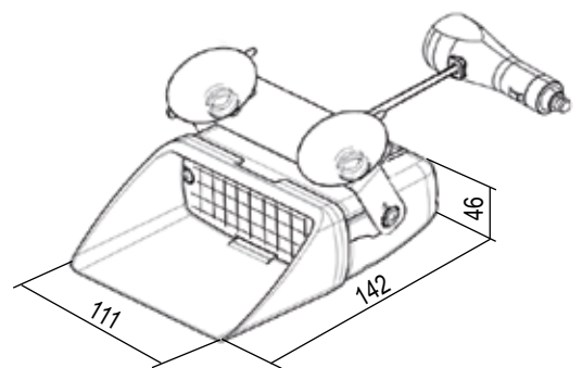
Viper S2 Solaris dimensions (mm).
